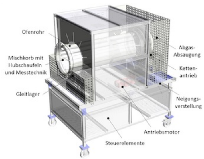
Thermoanalytisches Labor
